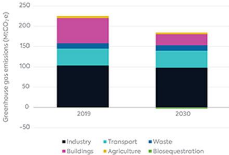
Figure 1: UAE's planned 2030 emissions reductions
